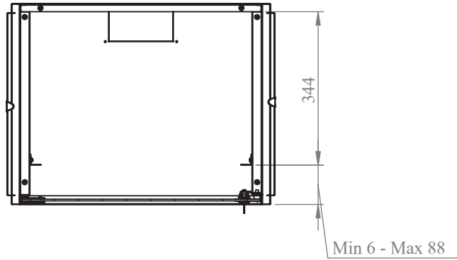
Max / min equipment mounting distance (450)
