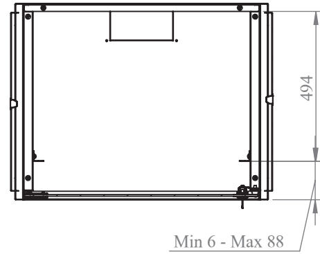
Max / min equipment mounting distance (600)
